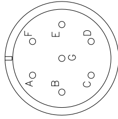
CABLE CONNECTOR
